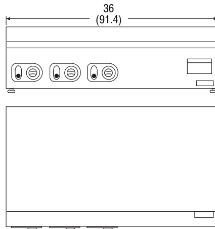
40717 Front and Top Views
