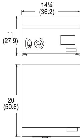
40715 Front and Top Views
